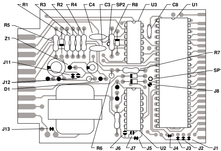
COMPONENT SIDE
