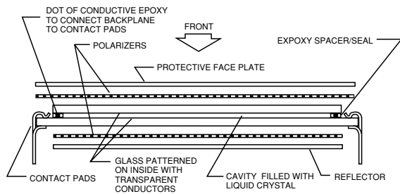
FIGURE 1. LCD Cross-Section
