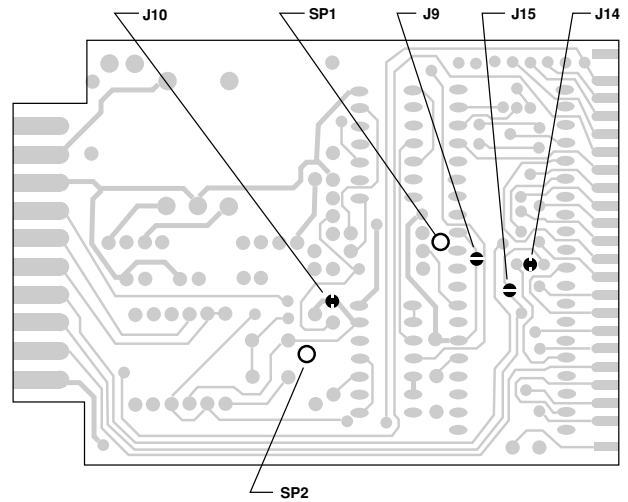
SOLDER SIDE
